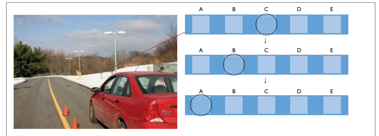
Figure 5: Test set-up at LRS. Detection targets simulating movement toward the street, creating a single moving target from discrete, temporally sequenced, targets
