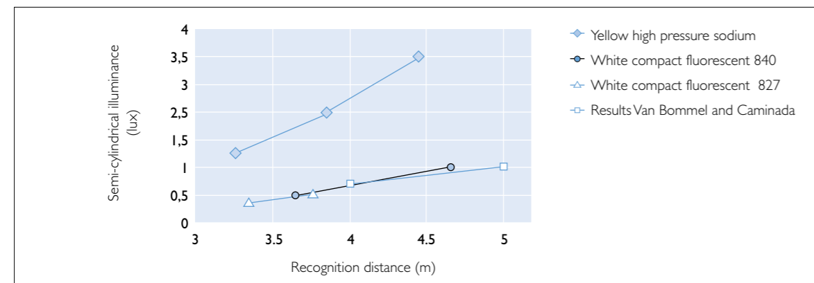
Figure 4: Facial recognition distance with different light sources (reproduced from Raynham)
