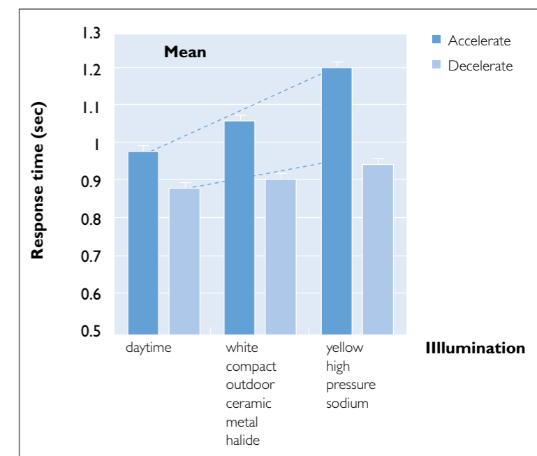
Figure 6: Response time with different light sources
