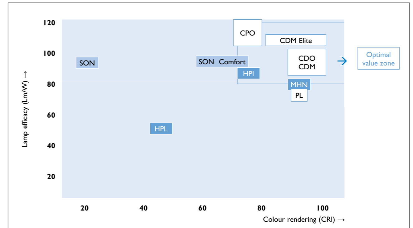
Figure 9: Colour rendering vs. lamp efficacy
