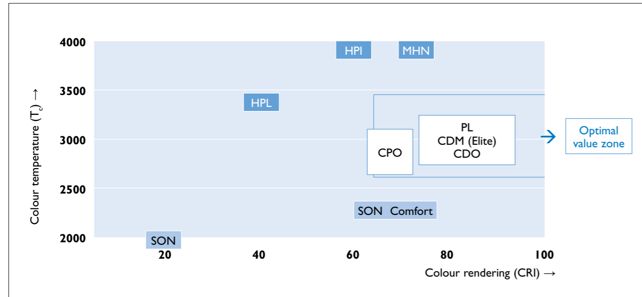
Figure 10: Colour temperature vs. colour rendering
